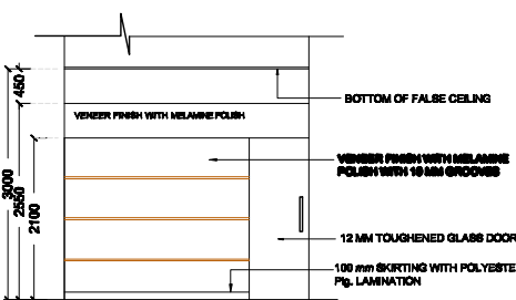
ELEVATION C
