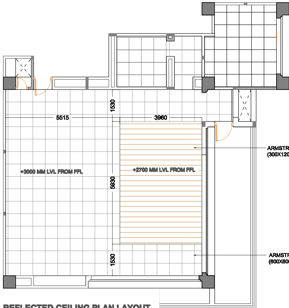
REFLECTED CEILING PLAN LAYOUT
